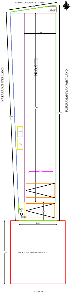
SITE PLAN
