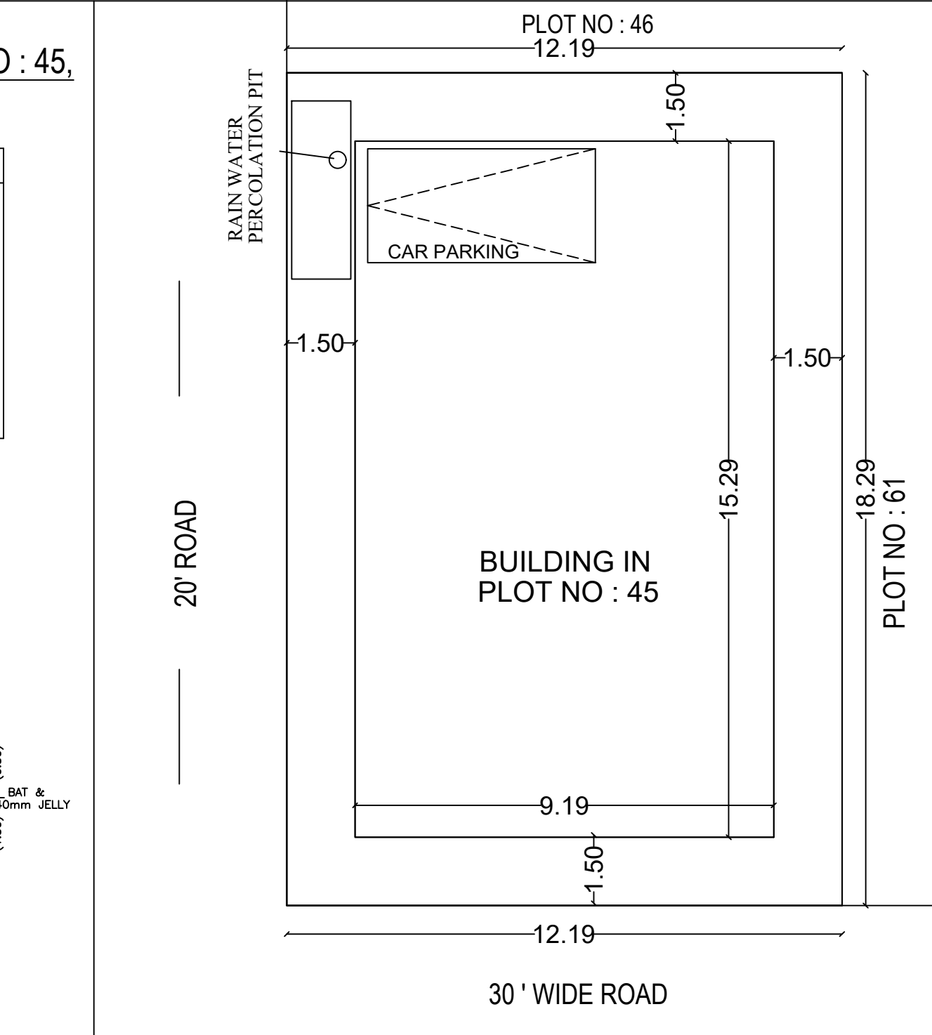
RAIN WATER HARVESTING SYSTEM
