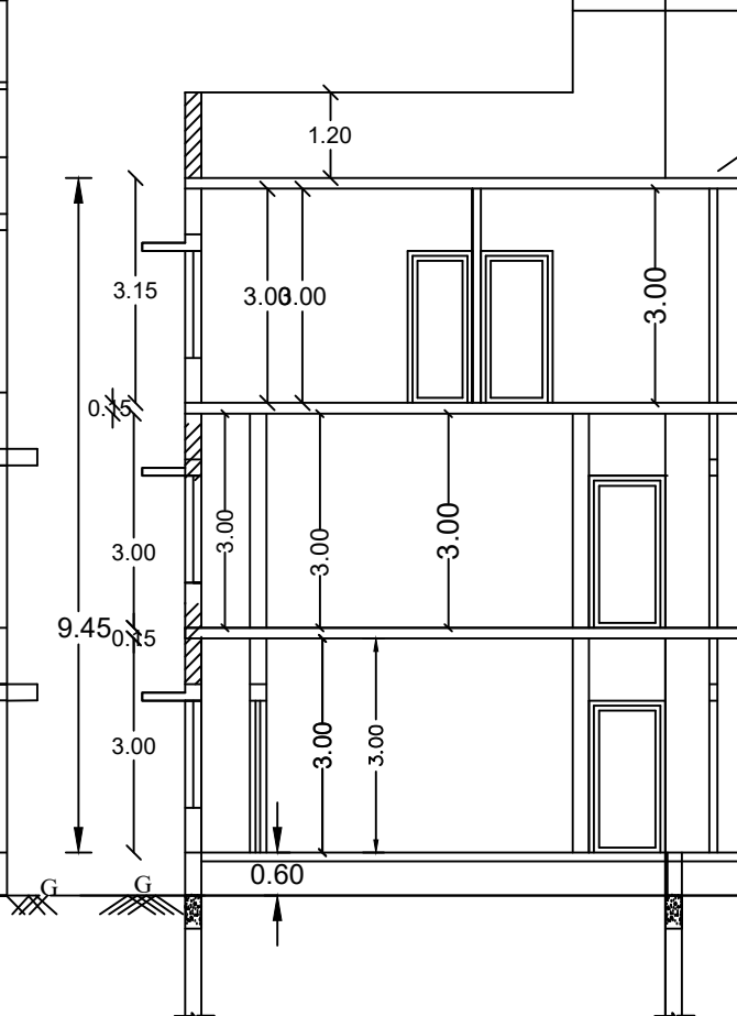
SECTION AA
