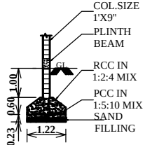
COLUMN DETAILS
