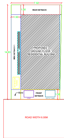
SITE PLAN
