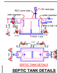
SEPTIC TANK DETAILS
