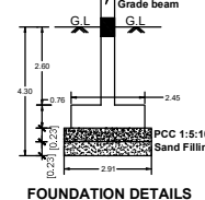
FOUNDATION DETAILS
