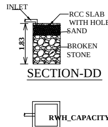
PLAN OF RWH
