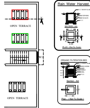
1st Floor Plan. Scale - 1:100 )
