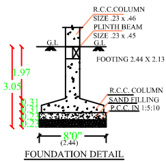
FOUNDATION DETAIL
