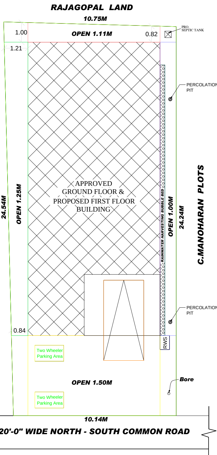
SITE PLAN (SCALE 1:1)
