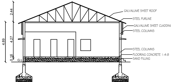
SECTION ON SS
