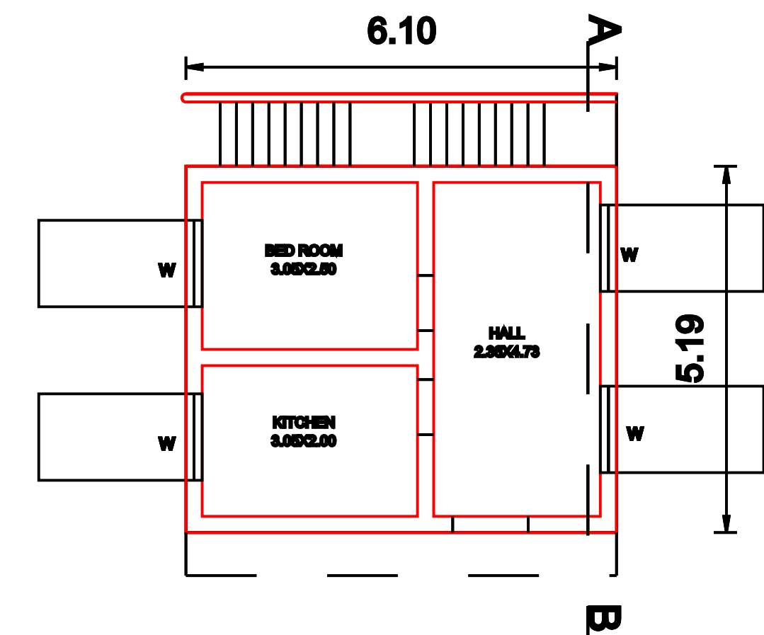
PROPOSED GROUND
