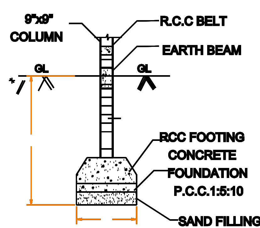
FOUNDATION DETAILS
