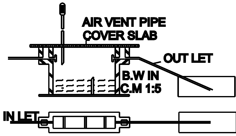
DETAILS OF SEPTIC TANK & D-TRENCE
