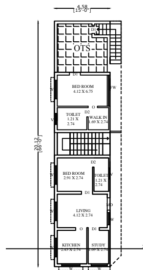
PRO. SECOND FLOOR PLAN
