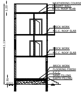
SECTION ON XX
