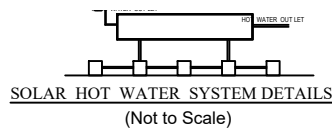
SOLAR SYSTEM
