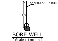
BORE WELL (Scale : 1m:4m)
