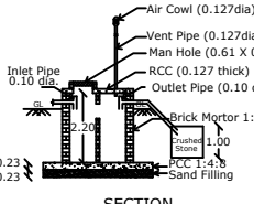
SECTION
