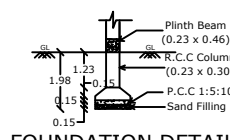
FOUNDATION DETAILS (Scale 1:100)
