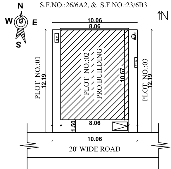
SITE PLAN ( SCALE: NTS)
