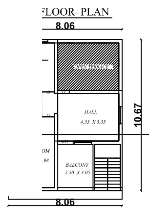
PRO. SECOND FLOOR PLAN
