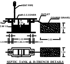
SEPTIC TANK & D-TRENCH DETAILS
