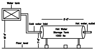
SOLAR WATER HEATER DETAILS
