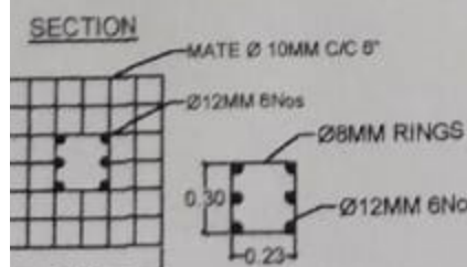
FOUNDATION DETAIL
