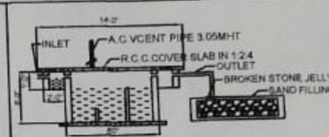
SECTION SEPTIC TANK & DISPERSION TRENCH
