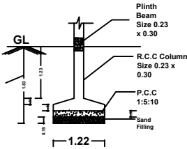
FOUNDATION DETAILS
