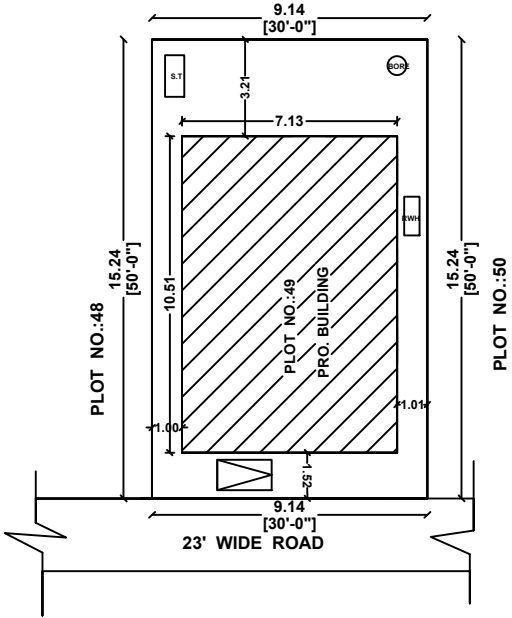
SITE PLAN
