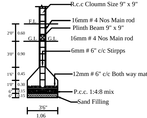
COLUMN DETIAL
