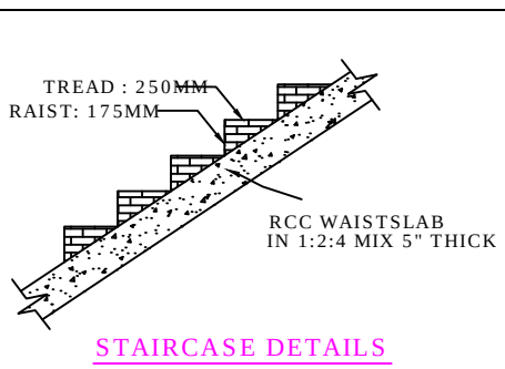
STAIRCASE DETAILS
