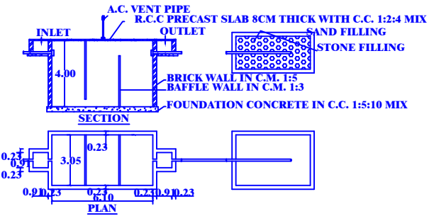
SEPTIC TANK & DISPERSION TRENCH
