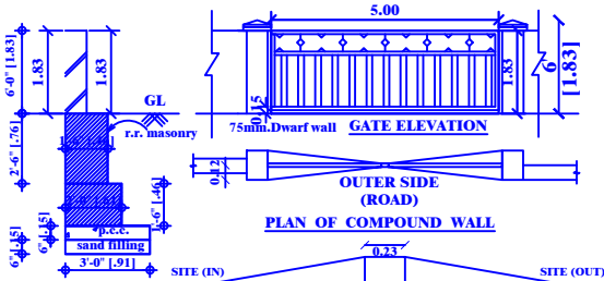
SECTION ON DWARF WALL (DW)
