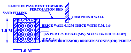
RAIN WATER SYSTEM
