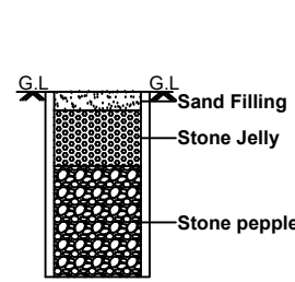
DETAILS OF RAIN WATER HARVESTING
