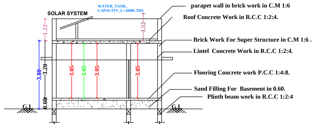
SECTION-AB
