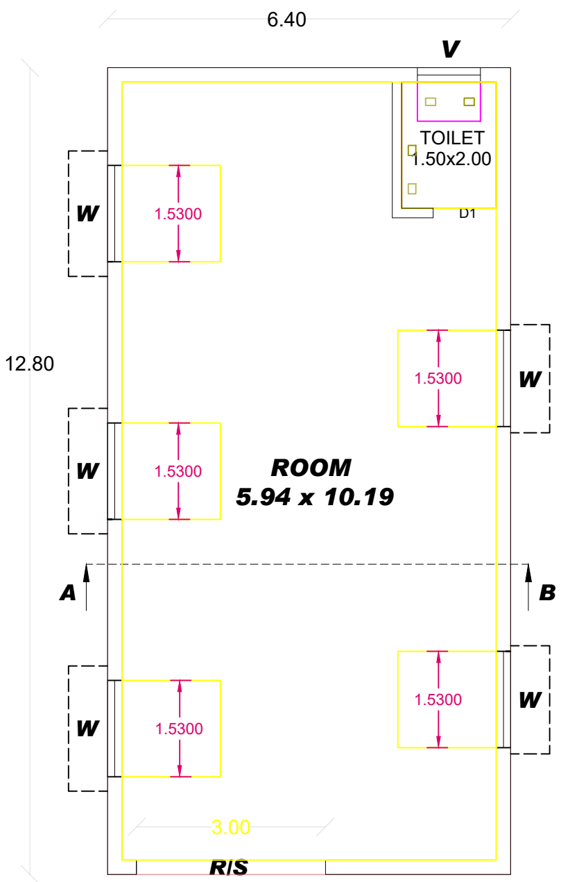
FLOOR PLAN
