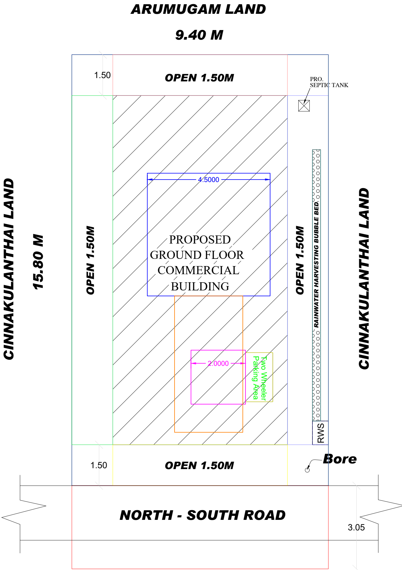
SITE PLAN
