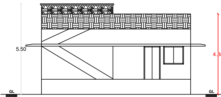
FRONT ELEVATION
