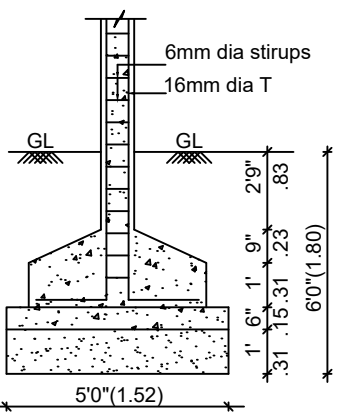
COLUMN FOUNDATION DETAIL SCALE (1:50)
