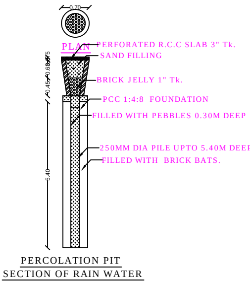
PERCOLATION PIT SECTION OF RAIN WATER
