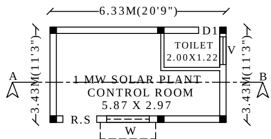
PRO.GROUND FLOOR PLAN (SOUTH FACING)
