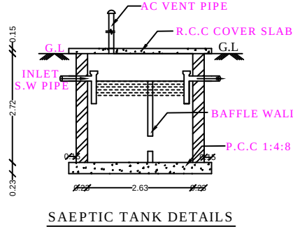
SAEPTIC TANK DETAILS
