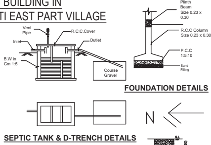
SEPTIC TANK & D-TRENCH DETAILS
