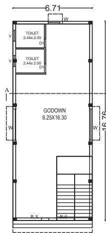
PRO.GROUND FLOOR PLAN
