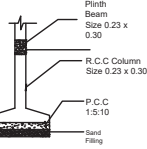
FOUNDATION DETAILS
