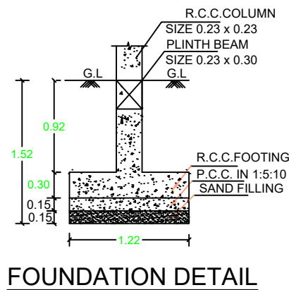
FOUNDATION DETAIL
