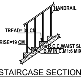
STAIRCASE SECTION
