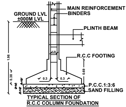
TYPICAL SECTION OF R.C.C COLUMN FOUNDATION
