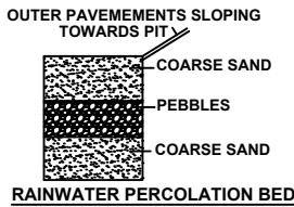
RAINWATER PERCOLATION BED
