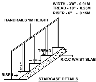
STAIRCASE DETAILS
