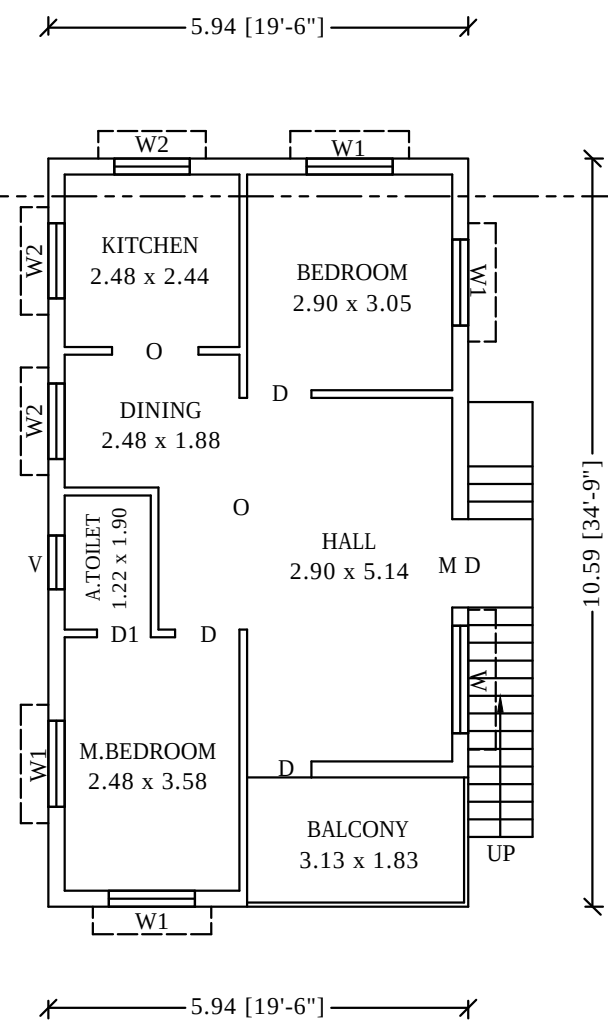
EXI.FIRST FLOOR PLAN
