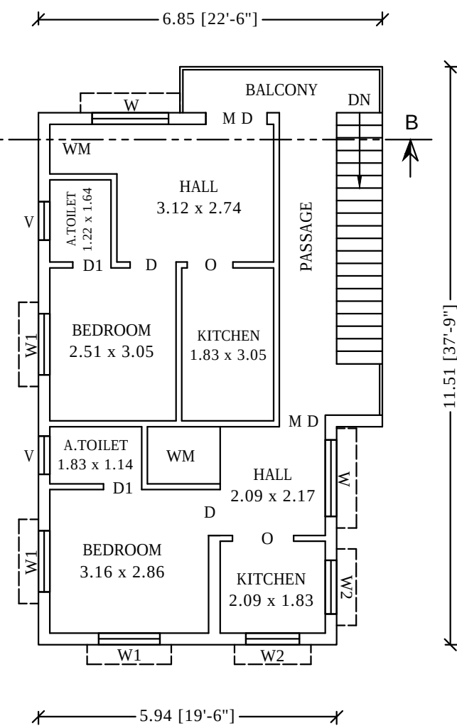
PRO.SECOND FLOOR PLAN
