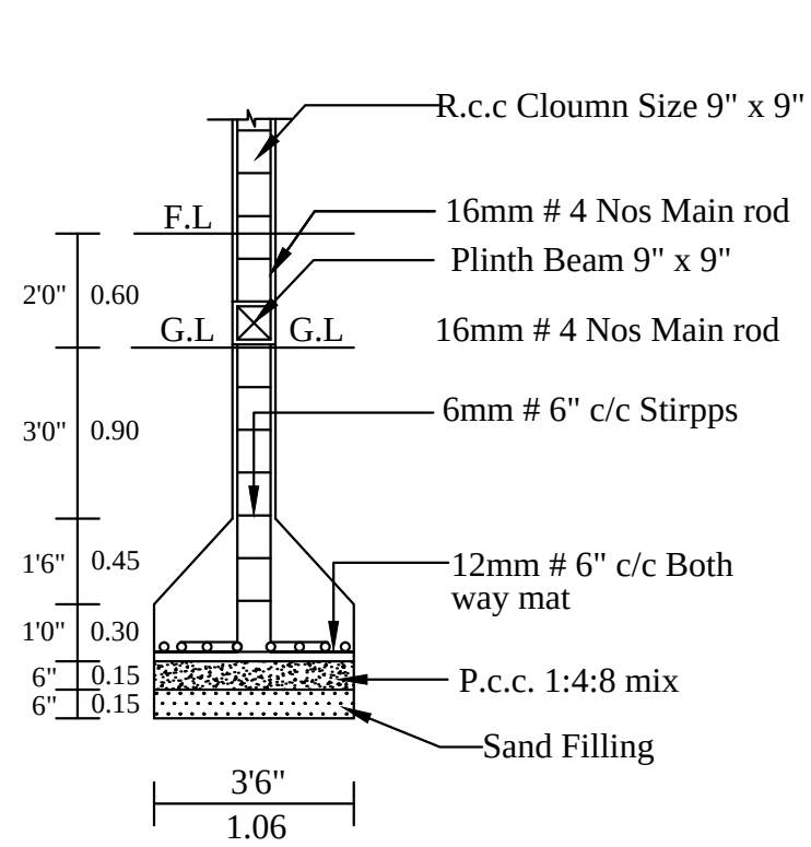
COLUMN DETIALS
