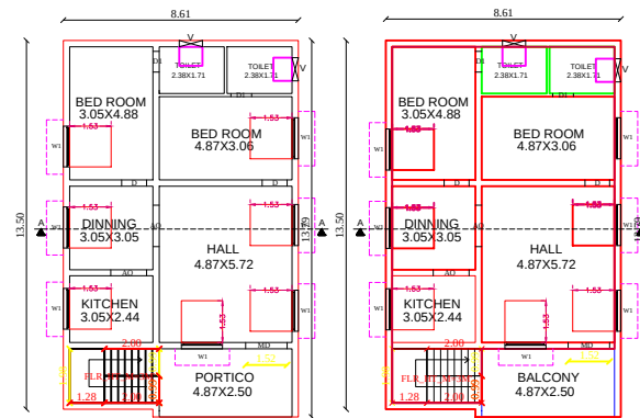
EXISTING FLOOR PLAN PROPOSED FIRST FLOOR PLAN
