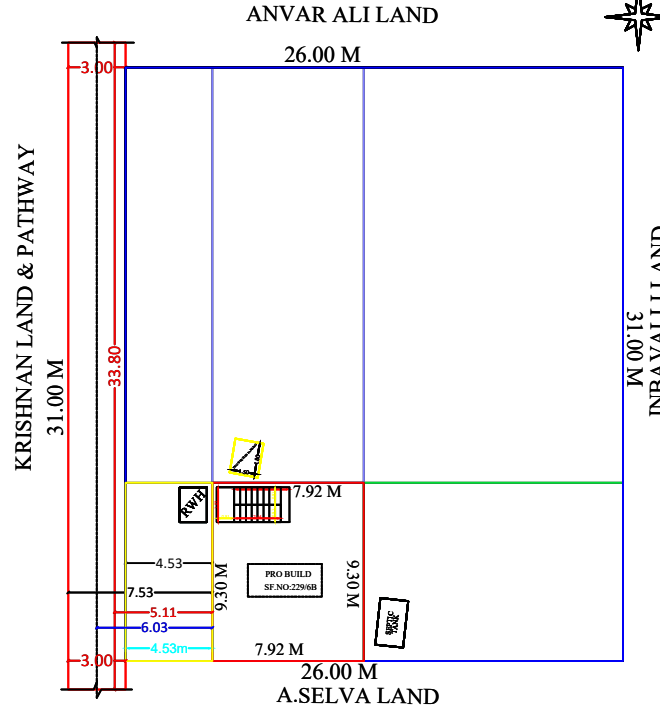
SITE PLAN (Not For Scale)
