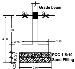
FOUNDATION DETAILS
