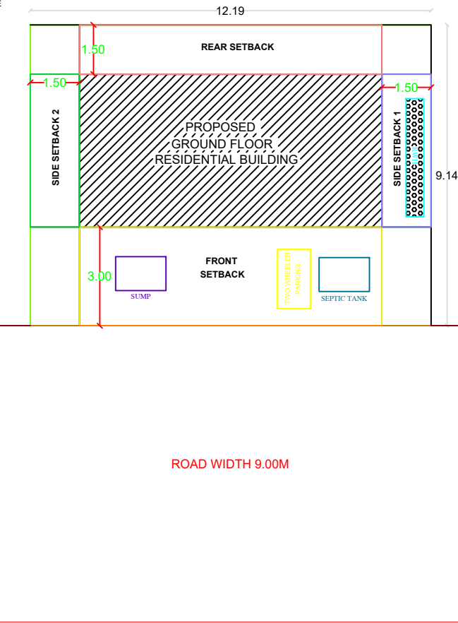
SITE PLAN
