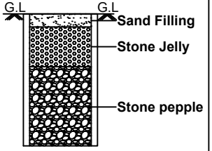
DETAILS OF RAIN WATER HARVESTING
