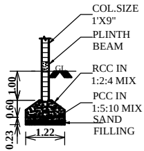
COLUMN DETAILS
