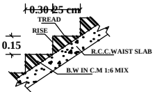
SECTION OF STAIRCASE
