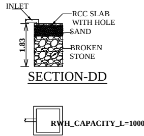
PLAN OF RWH
