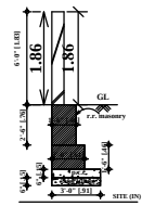
COMPOUND WALL
