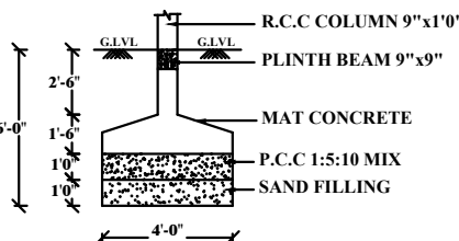
COLUMN FOUNDATION (NOT TO SCALE)
