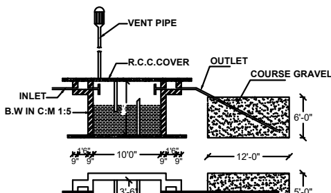
SEPTIC TANK & D-TRENCH DETAILS (NOT TO SCALE)
