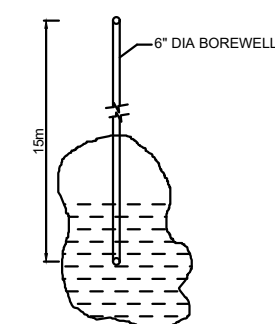
BORE WELL DETAIL
