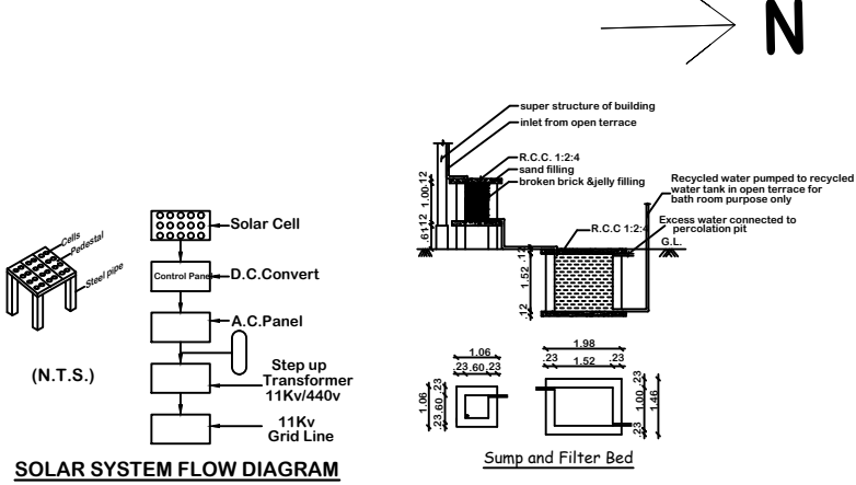
SOLAR SYSTEM FLOW DIAGRAM
