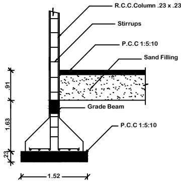
COLUMN DETAIL
