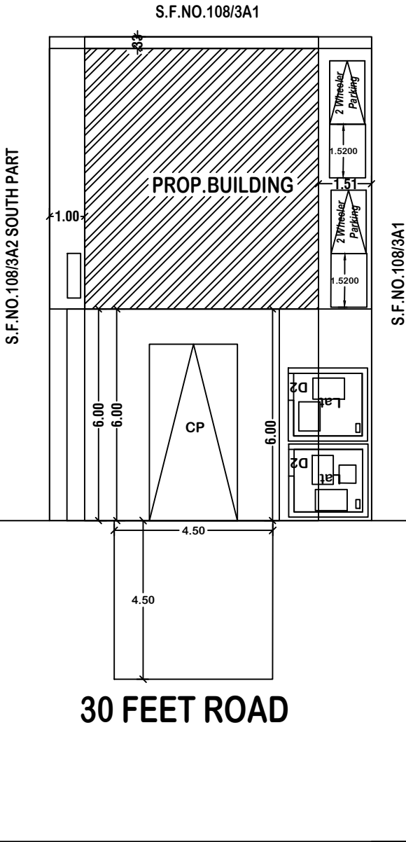
SITE PLAN
