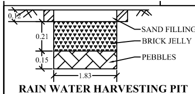
RAIN WATER HARVESTING PIT
