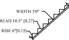
STAIR CASE DETAIL
