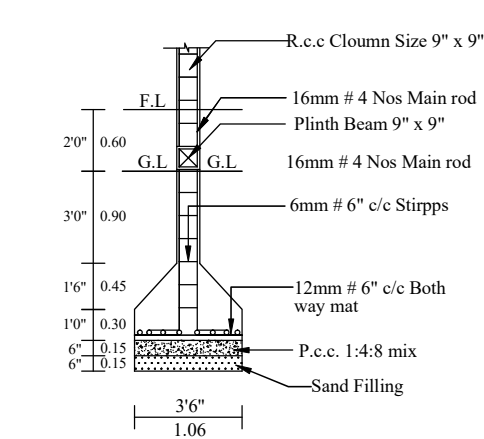
COLUMN DETAILS
