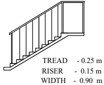
STAIRCASE DETAILS
