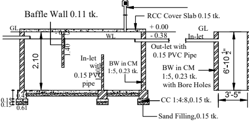
SECTION - SEPTIC TANK & SOAK PIT
