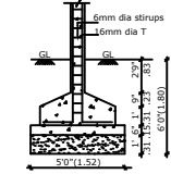
COLUMN FOUNDATION DETAIL
