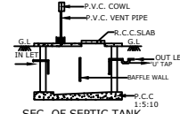
SEC. OF SEPTIC TANK
