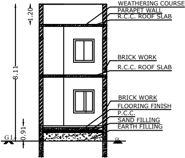
SECTION ON XX
