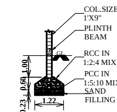
COLUMN DETAILS
