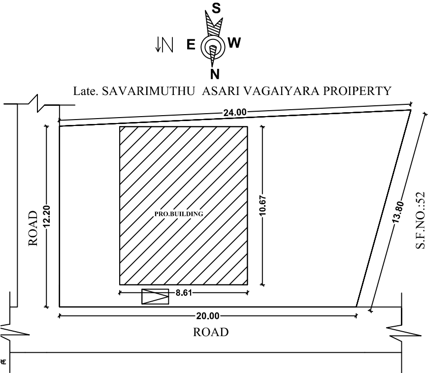
SITE PLAN
