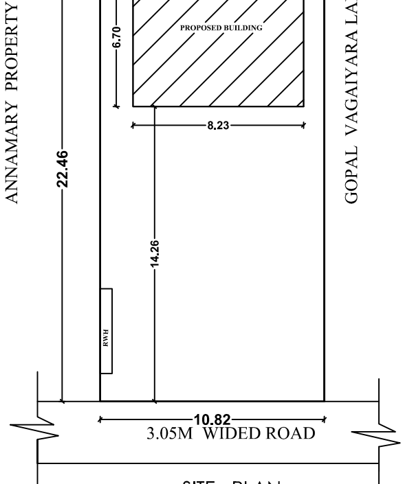
SITE PLAN
