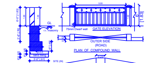
COMPOUND WALL DETAIL SECTION ON DWARF WALL
