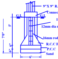
FOUNDATION DETAILS
