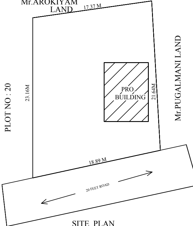
SITE PLAN
