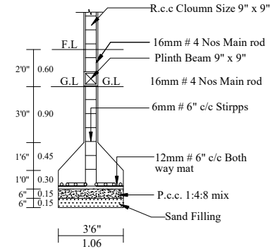
COLUMN DETAILS
