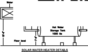
SOLAR WATER HEATER DETAILS
