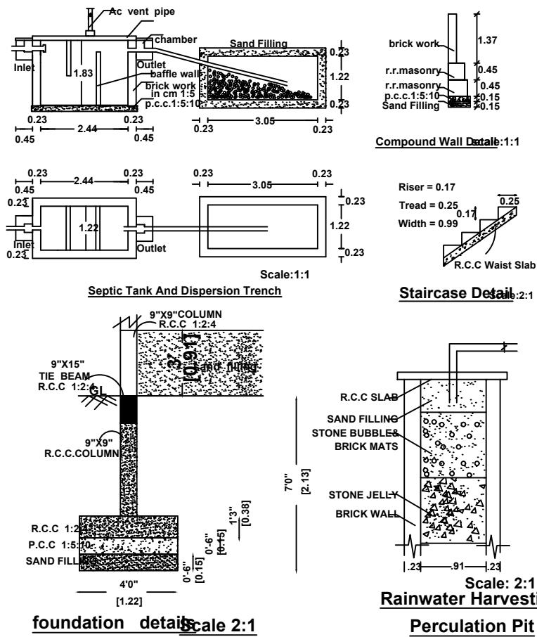
foundation details Scale 2:1
