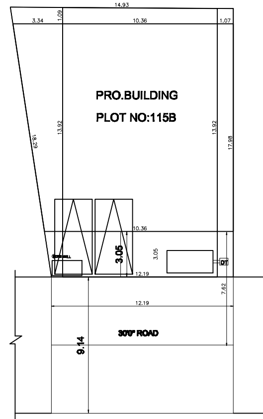
SITE PLAN
