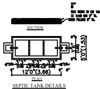
SEPTIC TANK DETAILS
