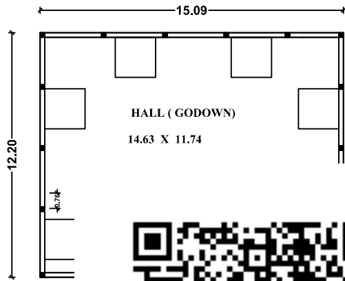
FLOOR PLAN
