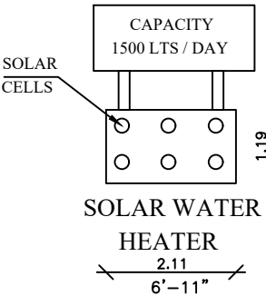
SOLAR PANEL
